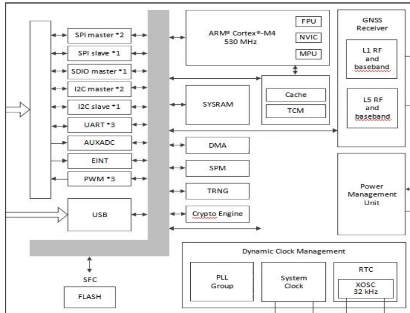
Figure 1: Block Diagram
