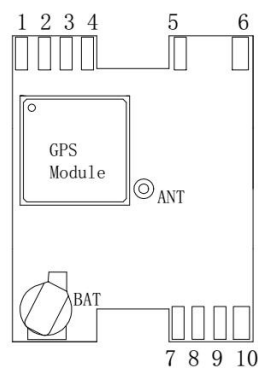
Figure 2: Pin Assignment
