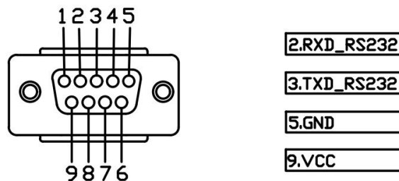
Figure 2: Pin Assignment
