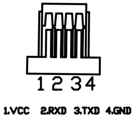
Figure 2: Pin Assignment
