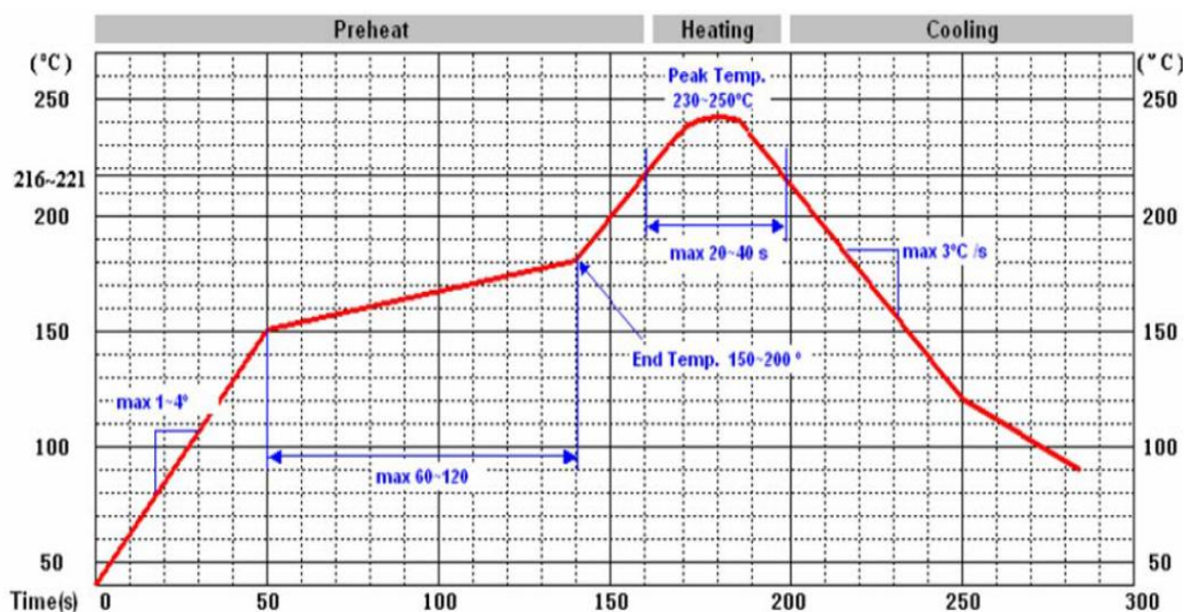
Figure 11: Recommended Reflow Soldering Thermal Profile
