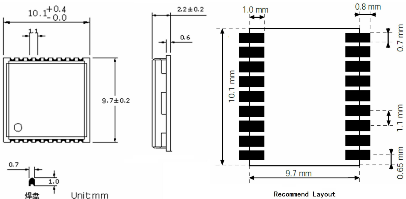
Figure 10: Bottom View Dimensions
