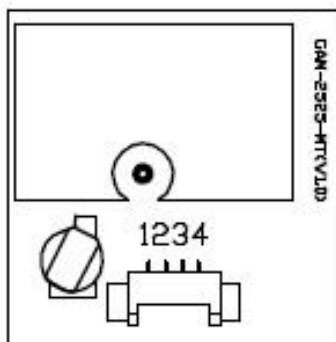
Figure 2: Pin Assignment
