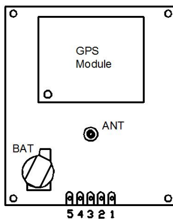
Figure 2: Pin Assignment
